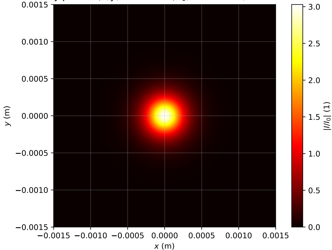
Intensity profile I(x, y, z = 3.582m)/I_0 , Pin=1.0Pcr, artificial time
